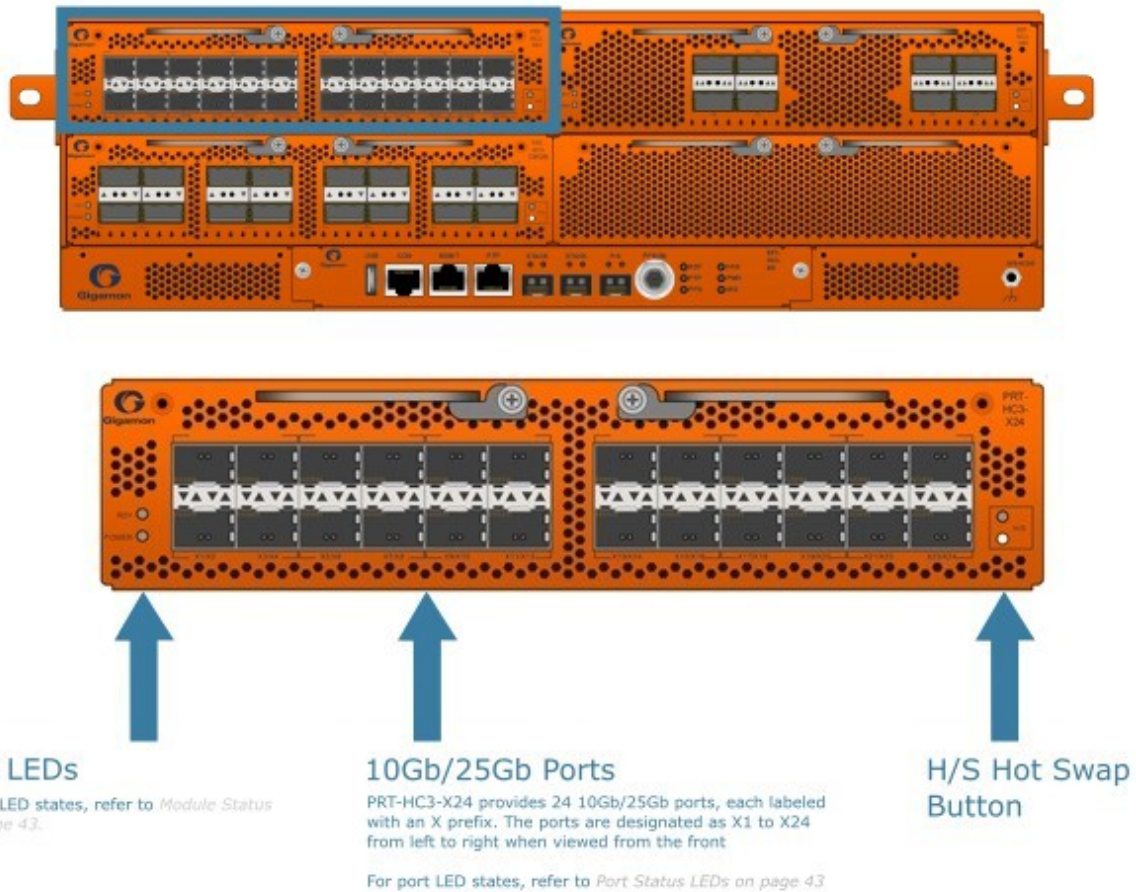
Figure 4 PRT-HC3-X24 Module
