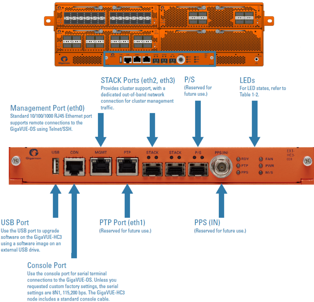
Figure 3 GigaVUE-HC3 Extension Board
