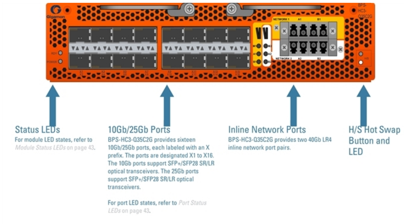
Figure 10 BPS-HC3-Q35C2G Module
